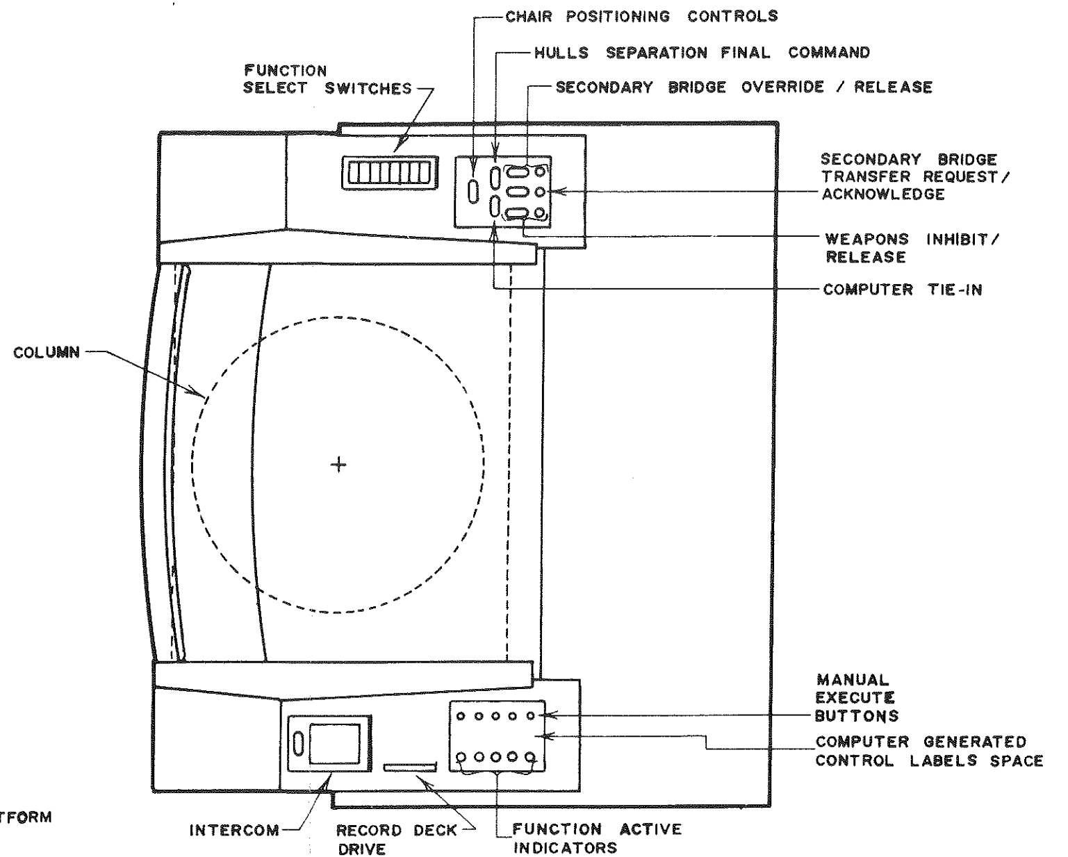
PLAN VIEW
